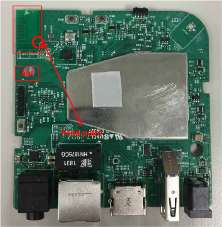
Figure 1. Antenna Placement
