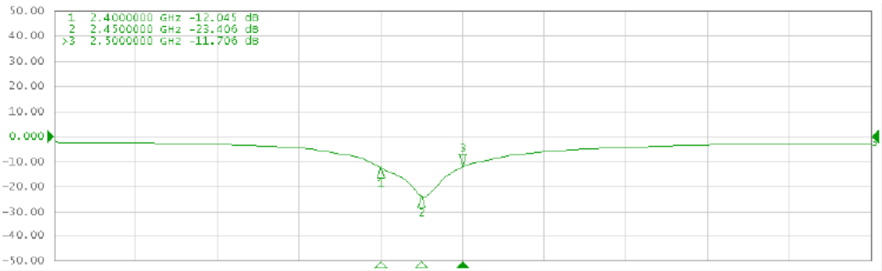
Figure 2. Antenna S-parameter
