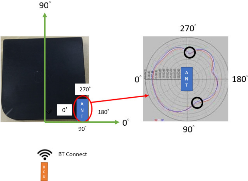
Figure 4. 2D Radiation Pattern
